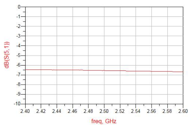
Figure 6. MQF2508G1 Coupling
