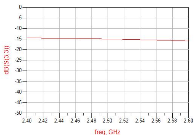
Figure 9. MQF2508G1 Return Loss (S33)
