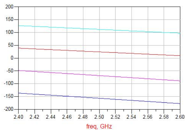
Figure 12. MQF2508G1 Phase
