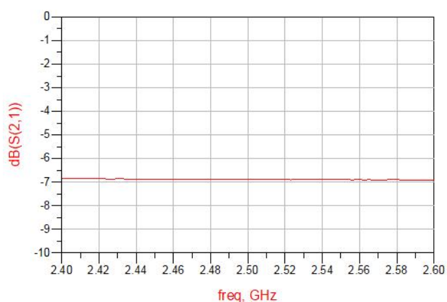
Figure 3. MQF2508G1 Coupling
