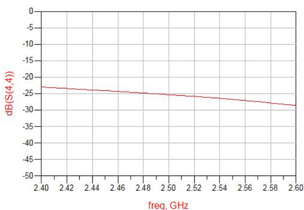
Figure 10. MQF2508G1 Return Loss (S44)
