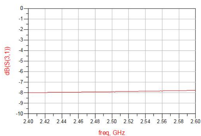
Figure 4. MQF2508G1 Coupling
