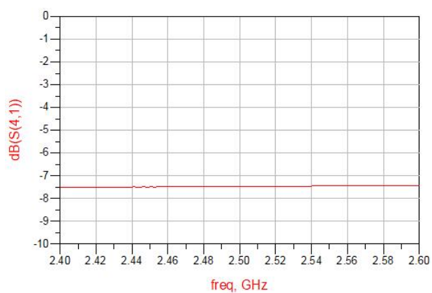
Figure 5. MQF2508G1 Coupling
