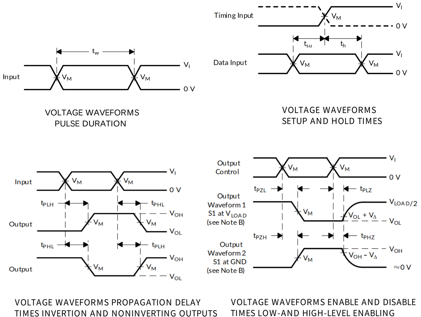
Figure 1. Load Circuit and Voltage Waveforms
