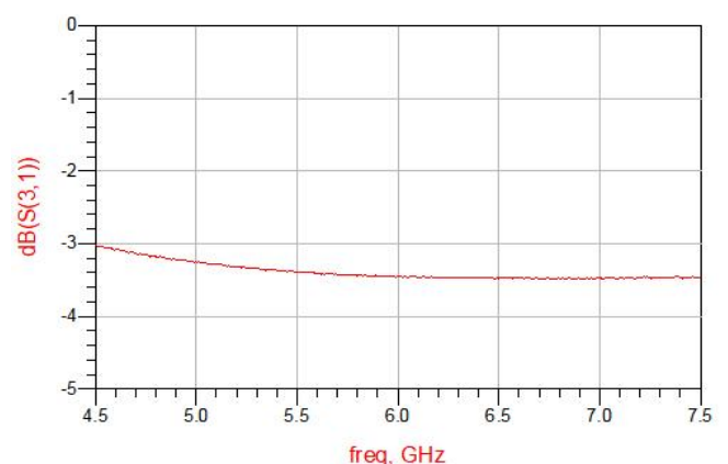
Figure 4. MHC60X03 Transmission
