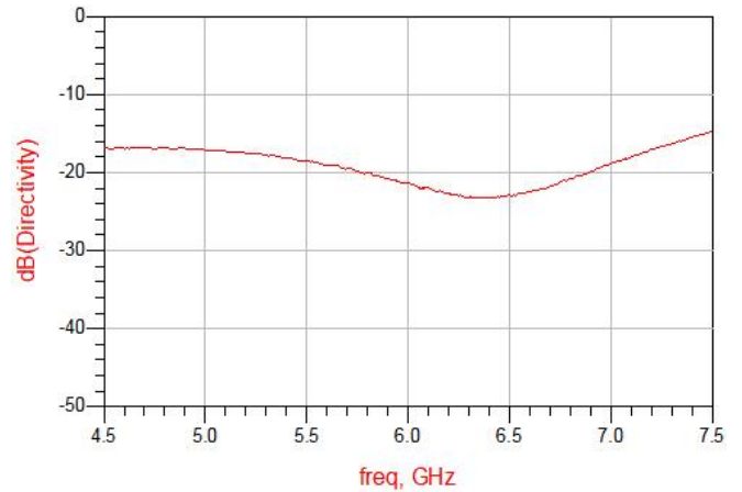
Figure 12. MHC60X03 Directivity
