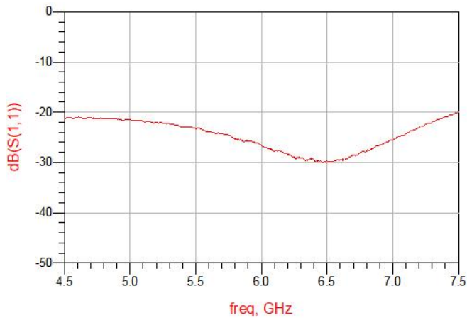
Figure 5. MHC60X03 Return Loss (S11)
