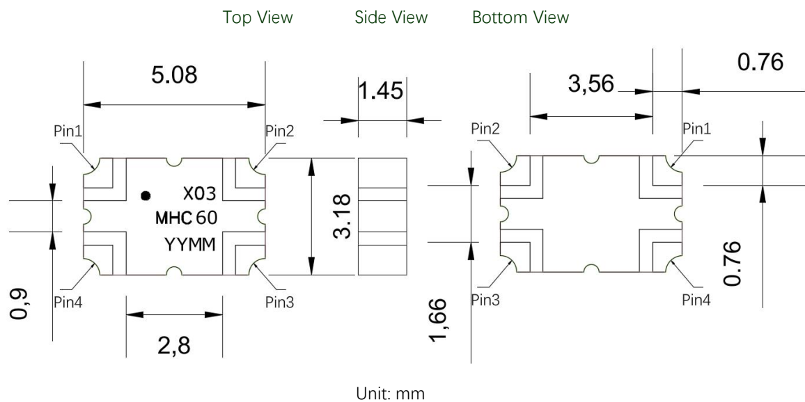
Figure 2. MHC60X03 Outline Drawing
