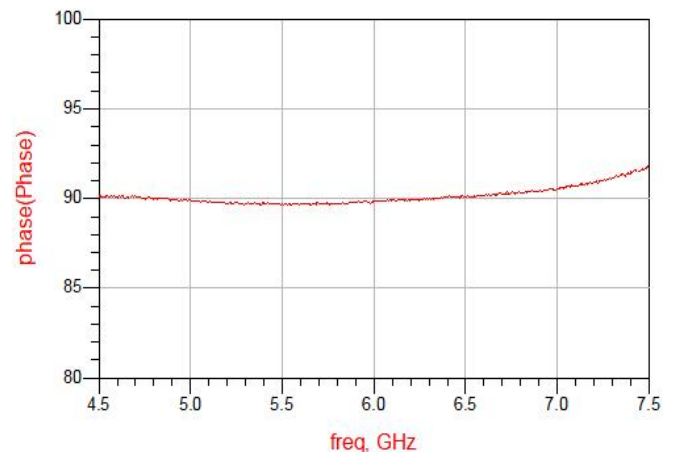
Figure 10. MHC60X03 Phase
