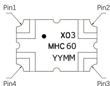
Figure 1. MHC60X03 (Top View)
