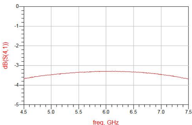
Figure 3. MHC60X03 Coupling
