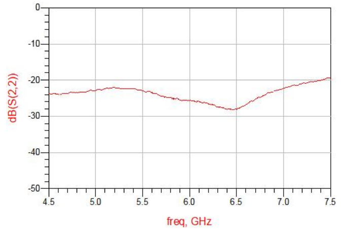
Figure 6. MHC60X03 Return Loss (S22)
