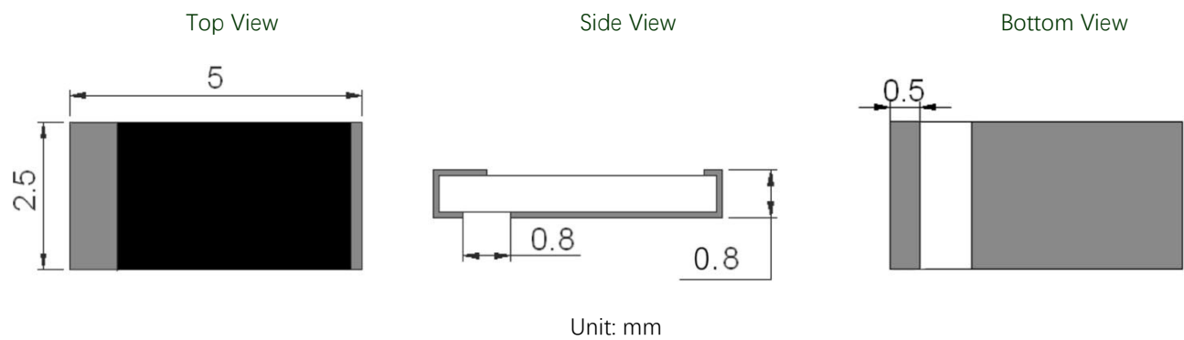
Figure1. MTE030X06 Outline Drawing
