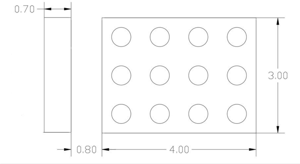
Figure 4. MTE030X06 Recommended PCB Layout
