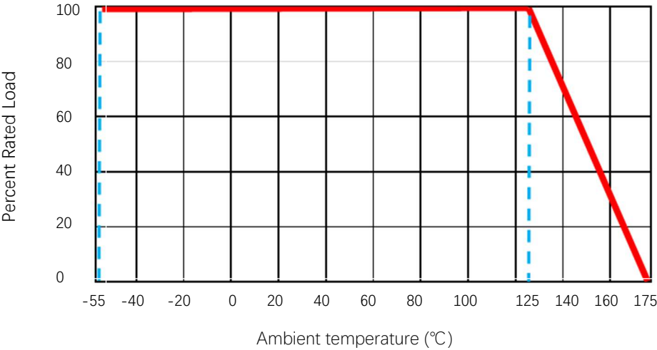
Figure 5. MTE030X06 Derating Curve
