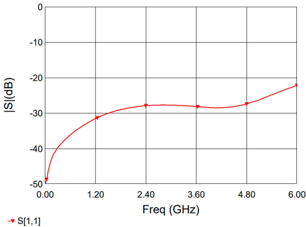
Figure 3. MTE020X06 Return Loss (S11)
