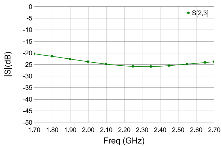
Figure 5. MPD1727W2 isolation
