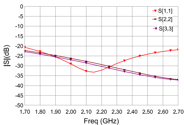
Figure 4. MPD1727W2 Return Loss
