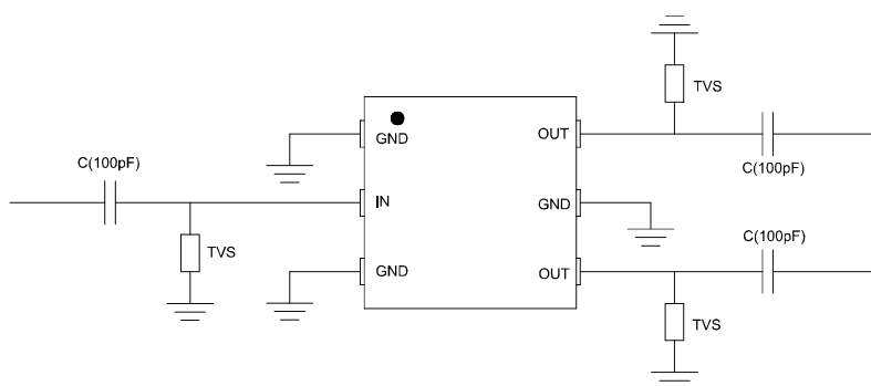
Figure 2. MPD1727W2 Suggested Circuits
