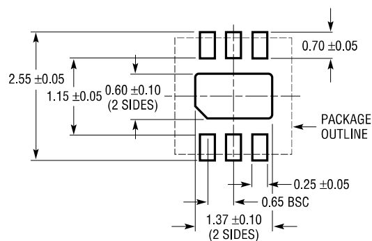
Figure 8. MPD1727W2 Recommended PCB Layout
