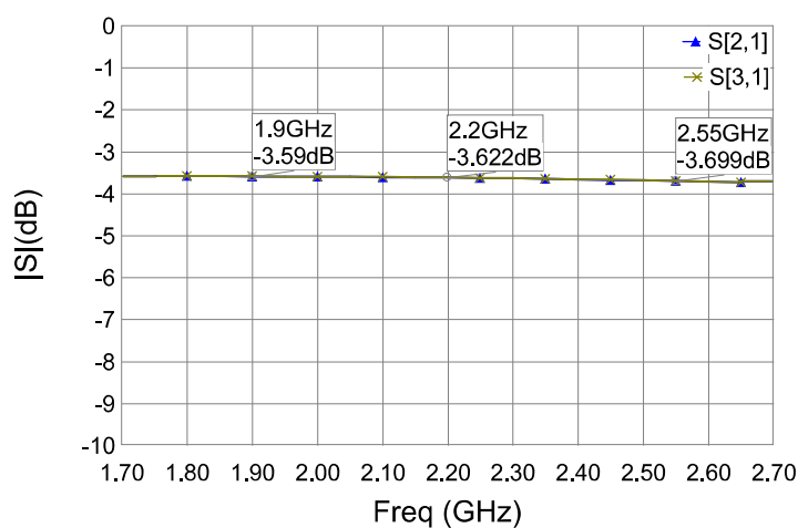
Figure 3. MPD1727W2 Insertion Loss
