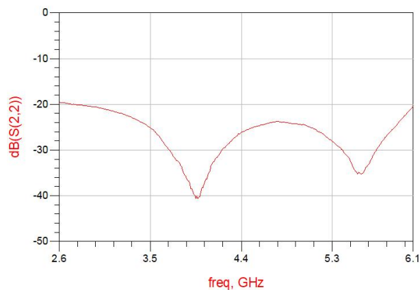
Figure 6. MHC4350L03 Return Loss (S22)
