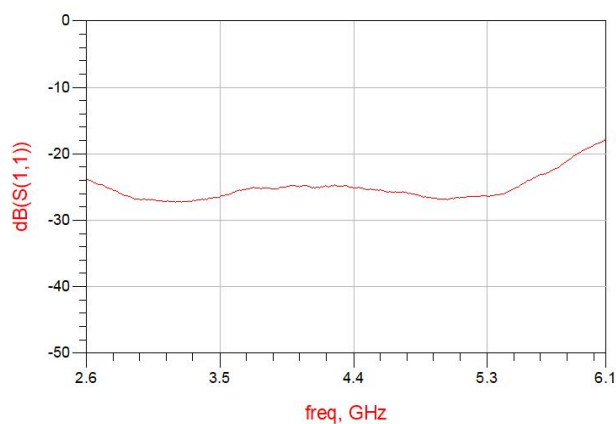
Figure 5. MHC4350L03 Return Loss (S11)
