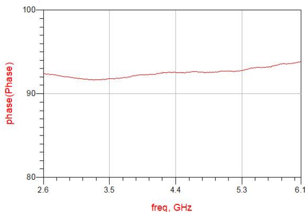
Figure 10. MHC4350L03 Phase
