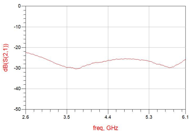
Figure 9. MHC4350L03 Isolation
