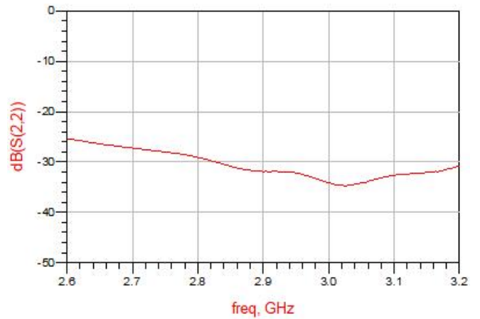
Figure 6. MHC29X03 Return Loss (S22)
