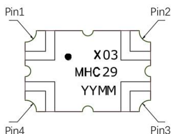
Figure 1. MHC29X03 (Top View)
