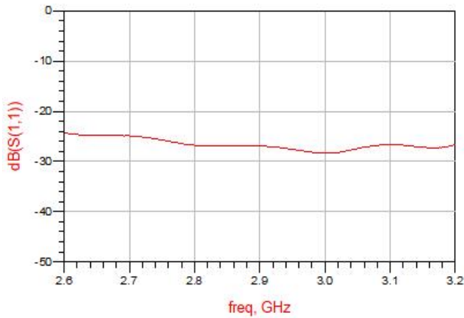
Figure 5. MHC29X03 Return Loss (S11)
