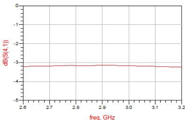
Figure 3. MHC29X03 Coupling
