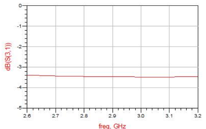
Figure 4. MHC29X03 Transmission
