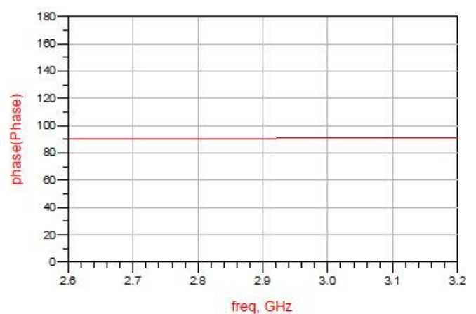
Figure 10. MHC29X03 Phase
