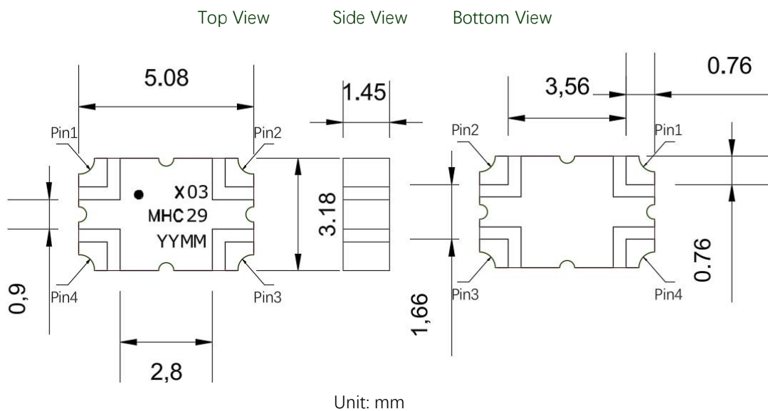
Figure 2. MHC29X03 Outline Drawing
