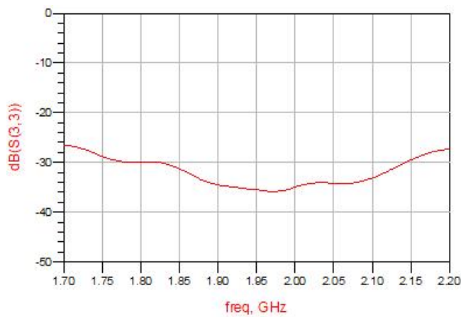
Figure 7. MHC21X02 Return Loss (S33)
