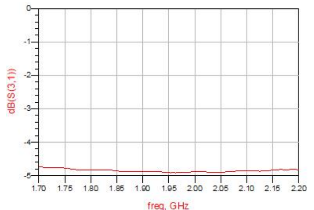
Figure 4. MHC21X02 Transmission
