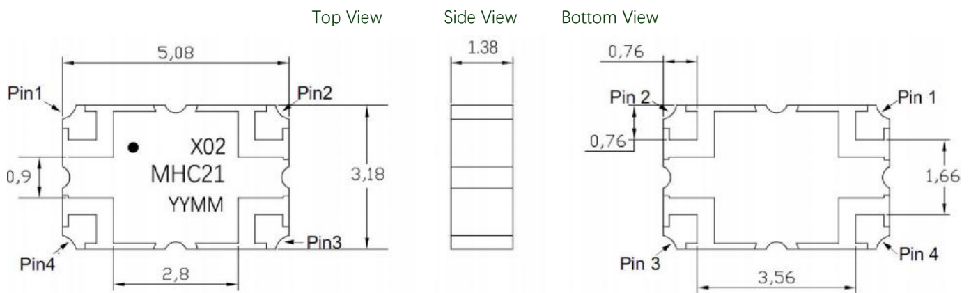
Figure 2. MHC21X02 Outline Drawing
