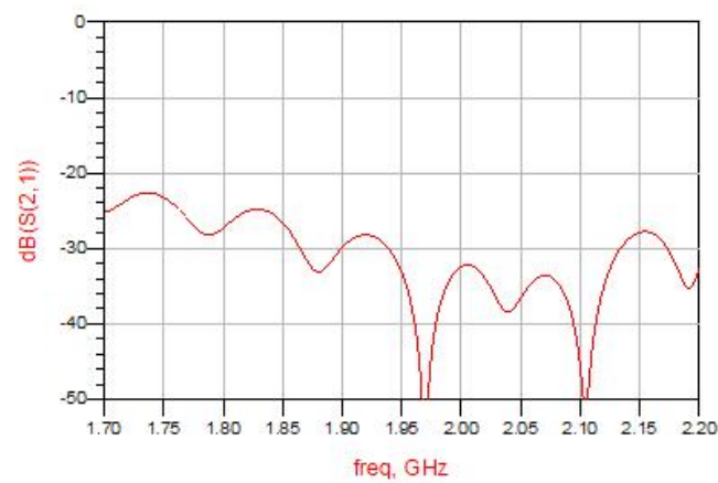
Figure 9. MHC21X02 Isolation
