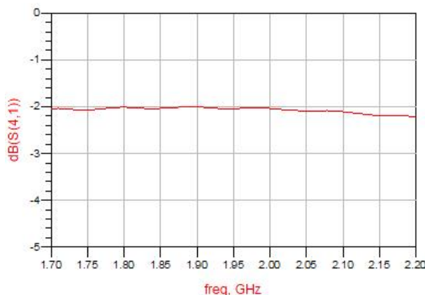
Figure 3. MHC21X02 Coupling
