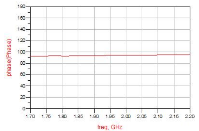
Figure 10. MHC21X02 Phase
