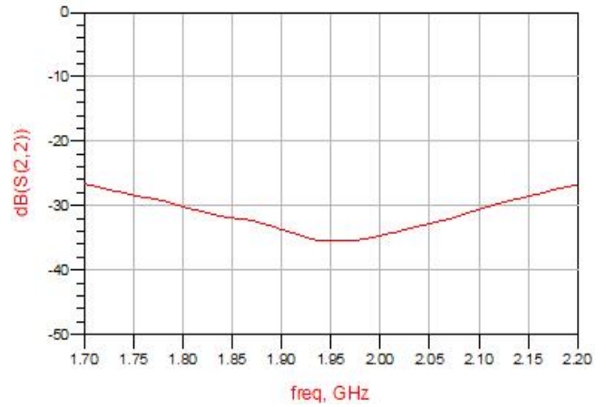
Figure 6. MHC21X02 Return Loss (S22)
