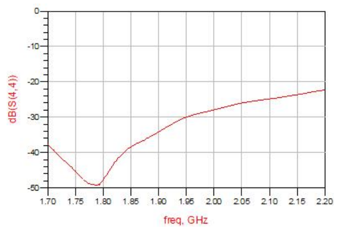
Figure 8. MHC21X02 Return Loss (S44)
