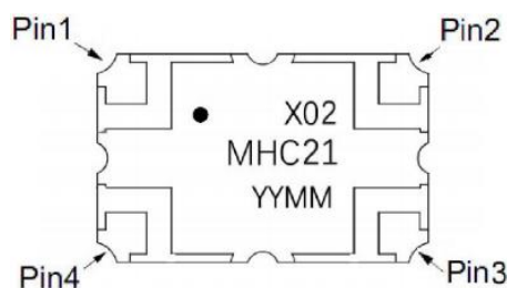
Figure 1. MHC21X02 (Top View)
