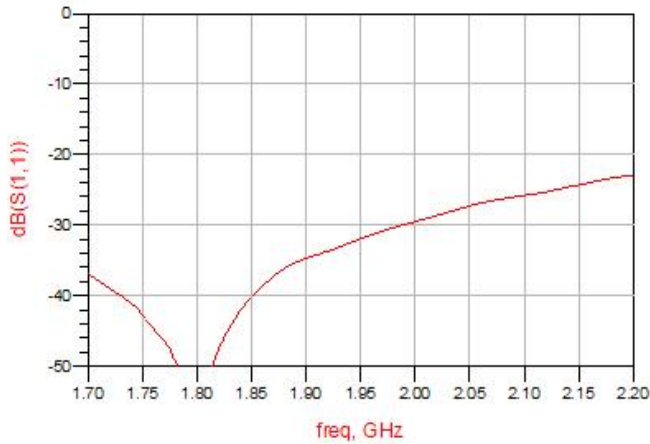
Figure 5. MHC21X02 Return Loss (S11)
