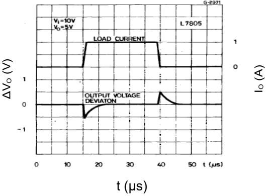
Figure 6: Load Transient Response
