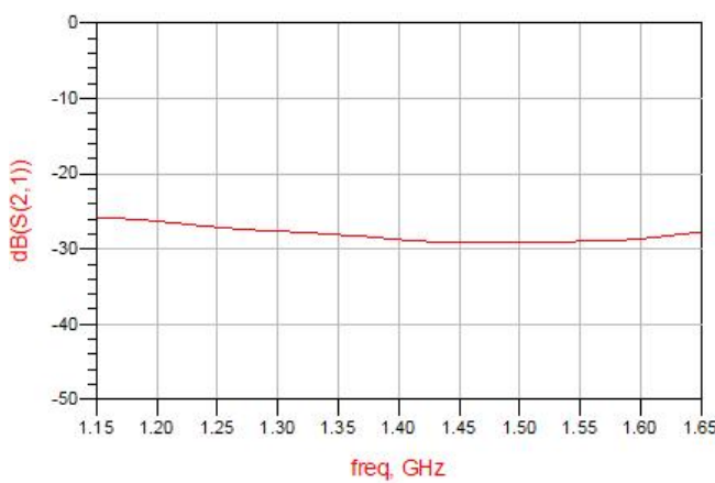
Figure 9. MHC1400C03 Isolation
