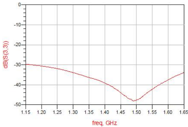
Figure 7. MHC1400C03 Return Loss (S33)
