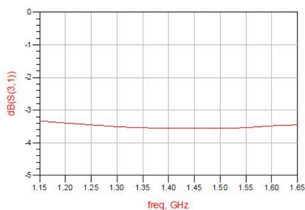
Figure 4. MHC1400C03 Transmission
