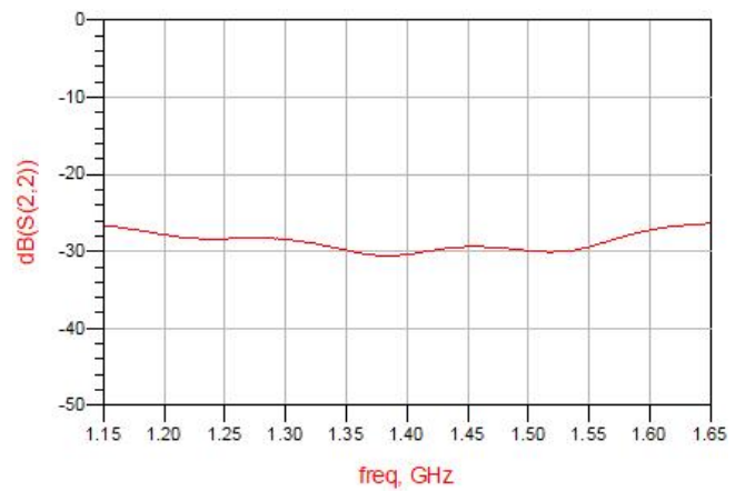
Figure 6. MHC1400C03 Return Loss (S22)
