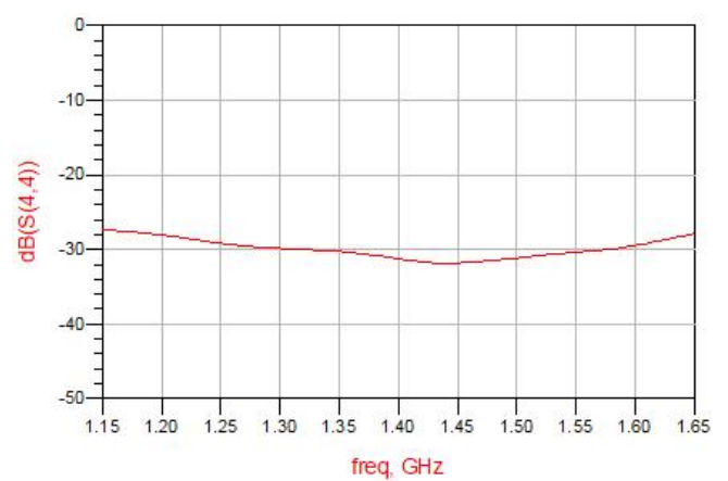
Figure 8. MHC1400C03 Return Loss (S44)
