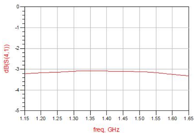
Figure 3. MHC1400C03 Coupling
