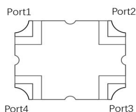
Figure 1. MHC1400C03 (Bottom View)
