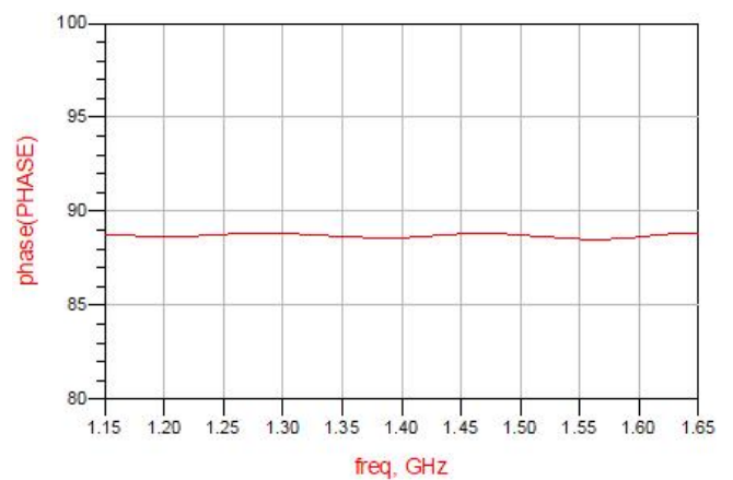
Figure 10. MHC1400C03 Phase
