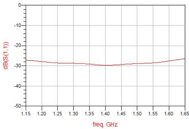
Figure 5. MHC1400C03 Return Loss (S11)
