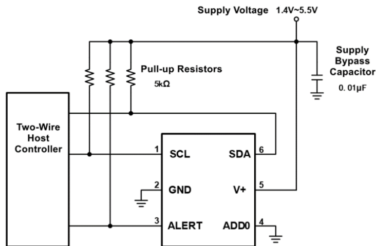
Figure 9. Typical Connections of the TMP102
