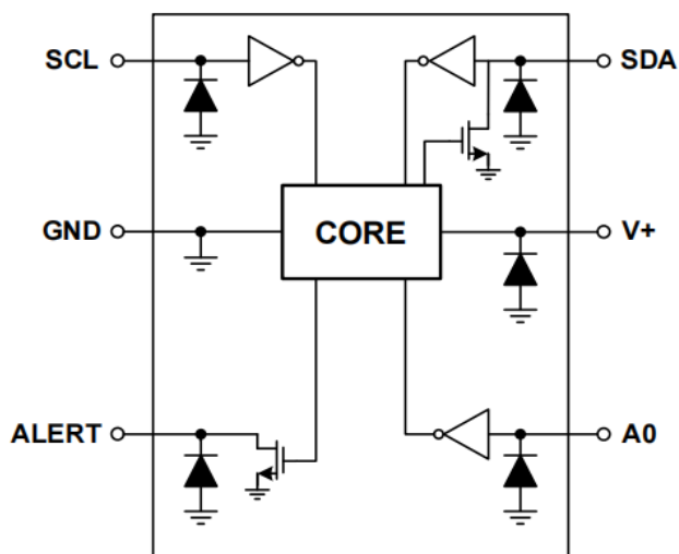
Figure 2. TMP102 Internal ESD Equivalent Circuit
