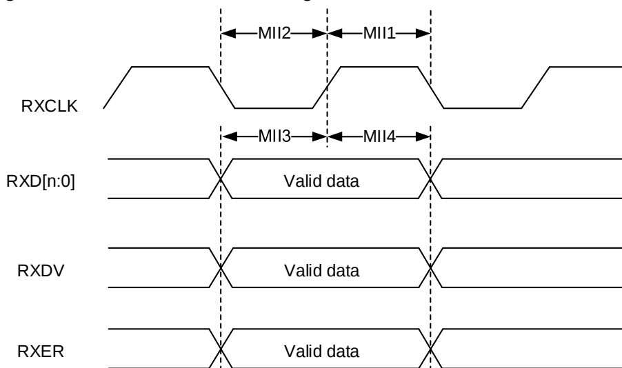
Figure 4-13. Ethernet MII receive diagram
