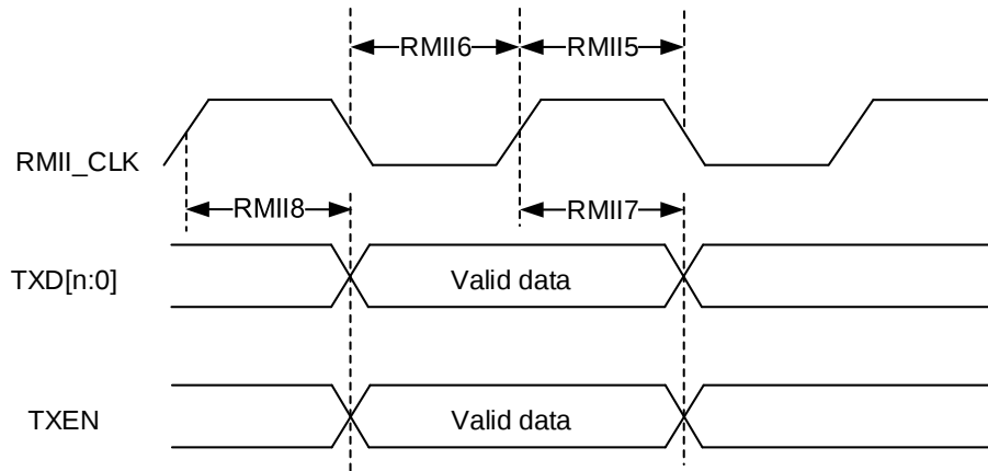
Figure 4-16. Ethernet RMII transmit diagram
