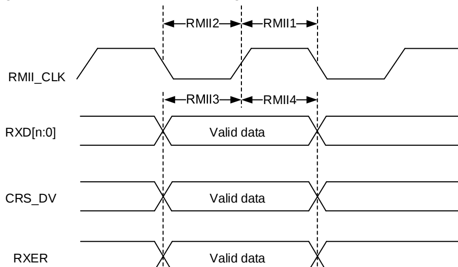
Figure 4-15. Ethernet RMII receive diagram
