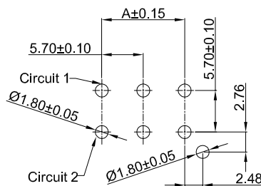
04-12Pin PCB REFERENCE DIAGRAM TOLERANCE:±0.05
