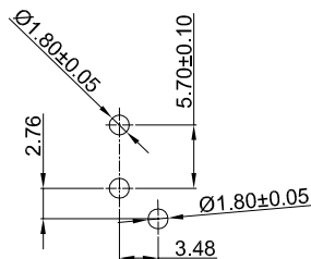
2Pin PCB REFERENCE DIAGRAM TOLERANCE:±0.05
