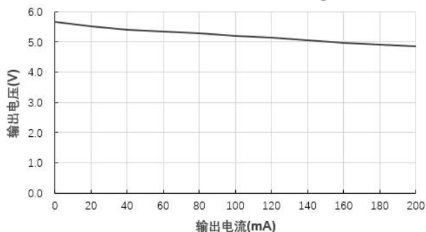
输出电压 VS 输出电流 B0305XT-1WR3@Vin=3.3V
