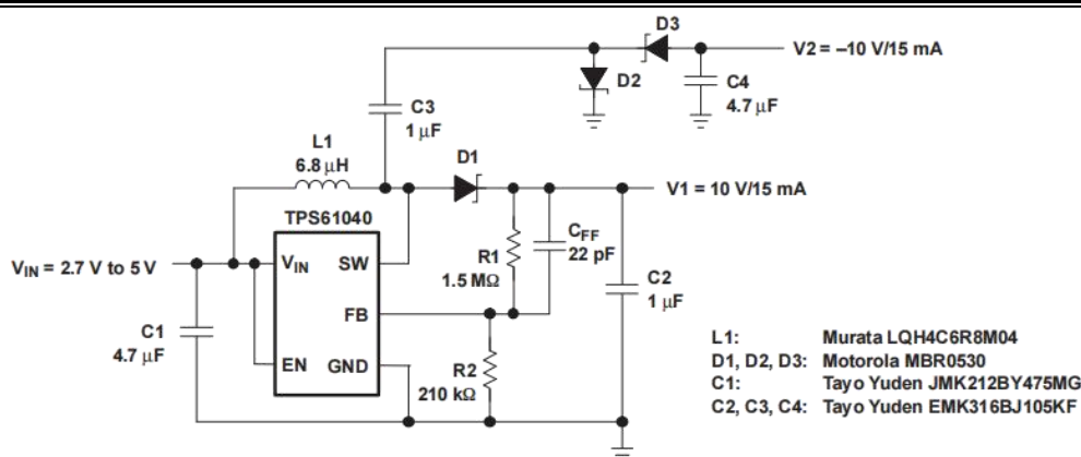
Figure 19. Positive and Negative Output LCD Bias Supply
