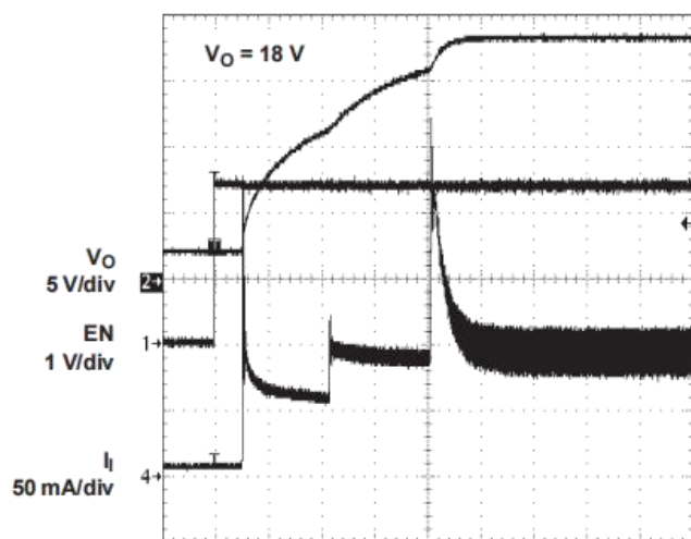
Figure 14. Start-Up Behavior
