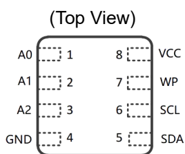
DFN-8 3*3/2*2
