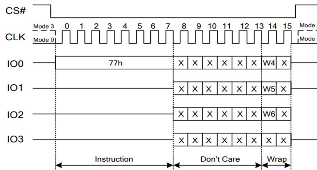
Figure 24 Set Burst with Wrap Instruction
