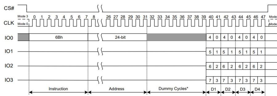
Figure 19 Fast Read Quad Output Instruction
