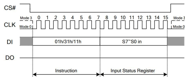
Figure 8 Write Status Register Instruction
