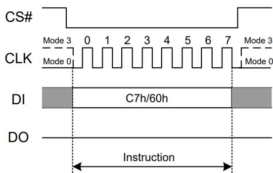
Figure 13 Chip Erase Instruction
