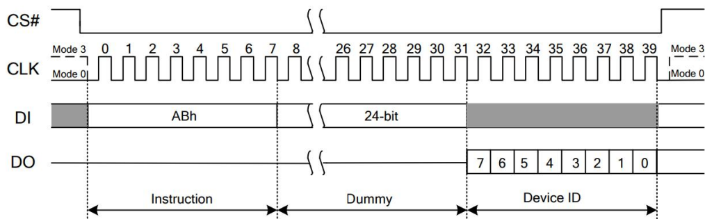
Figure 28 Release Power-down / Device ID
