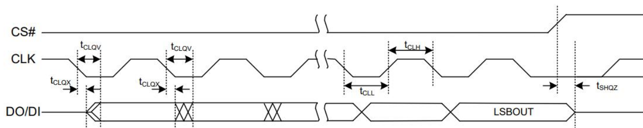
Figure 39 Serial Output Timing
