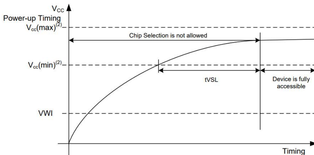
Figure 36 Power-up Timing
