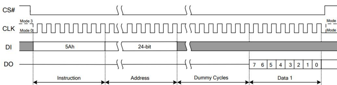
Figure 31 Read SFDP Register Instruction
