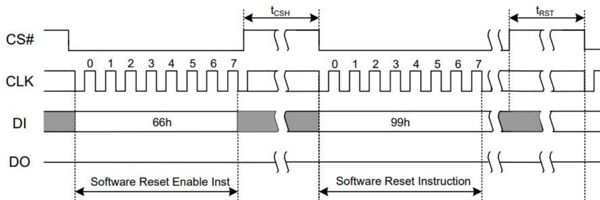
Figure 41 Software Reset Input Timing
