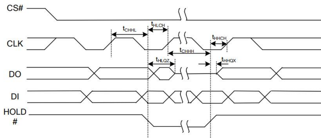
Figure 40 Hold Timing
