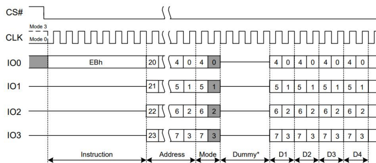
Figure 22 Fast Read Quad I/O Instruction(Initial command or previous M5-4 ≠10)
