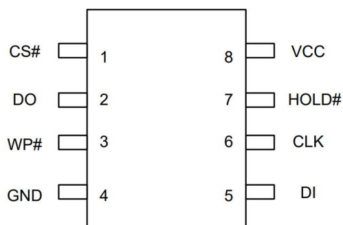
Figure 2 SOP-8 (150/208mil)/DFN-8
