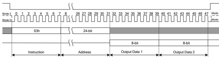
Figure 16 Read Data Instruction
