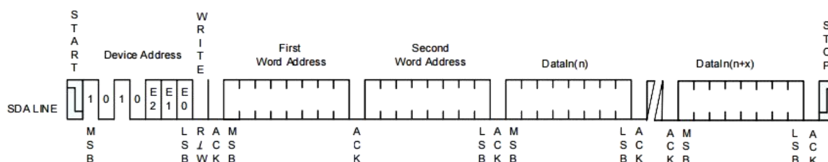
Figure 5-2 Page Write
