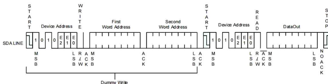
Figure 5-4 Random Read
