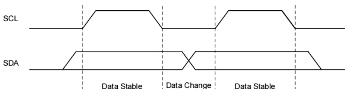
Figure 4-1 Data Validity
