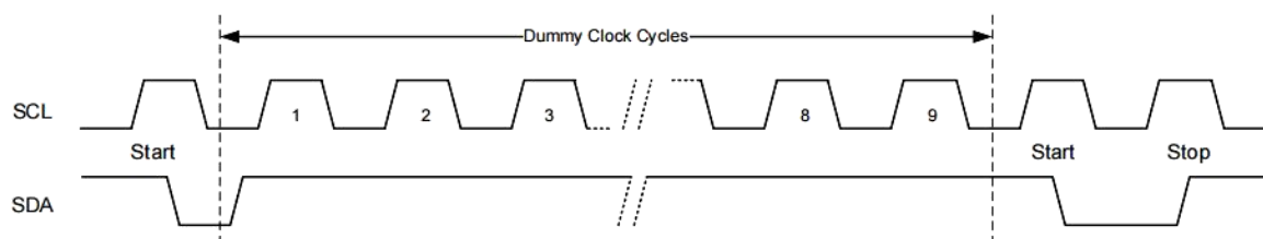
Figure 4-4 Soft Reset
