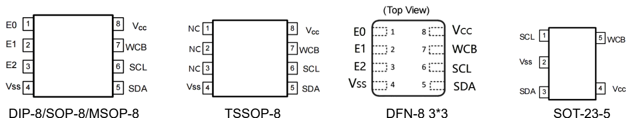
Figure 1-1 Pin Configuration
