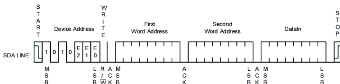
Figure 5-1 Byte Write
