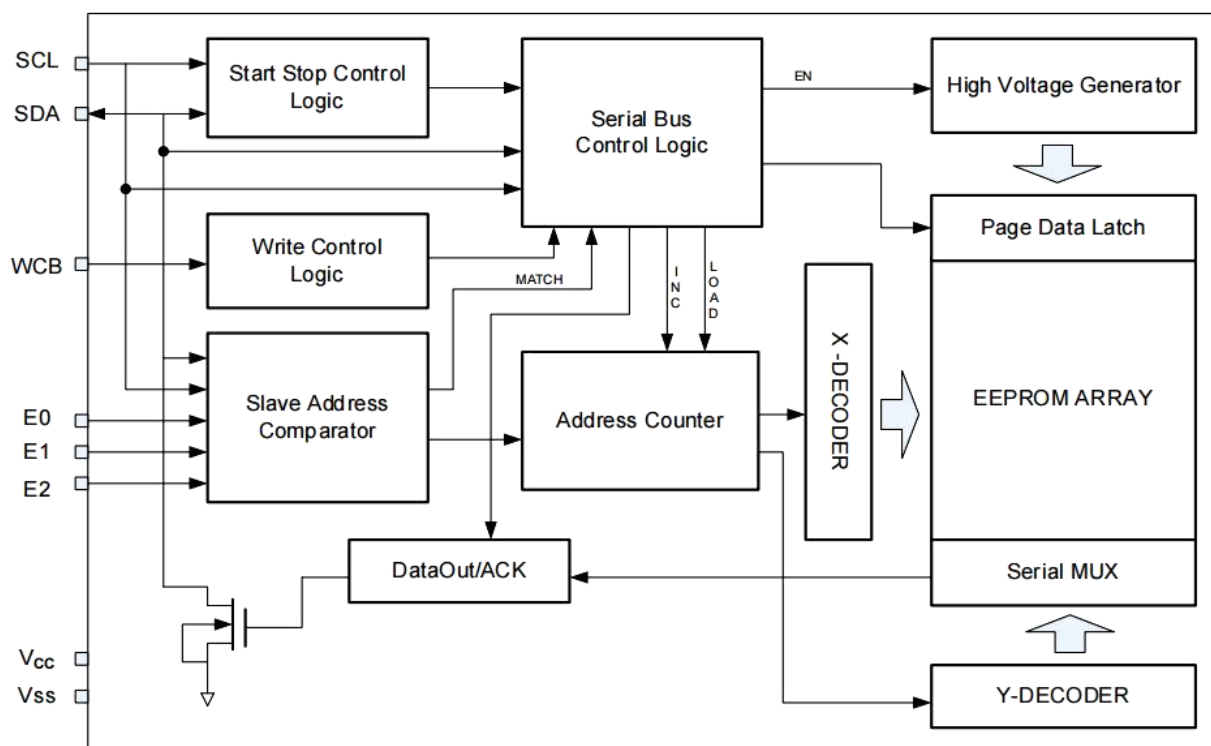
Figure 2-1 Block Diagram
