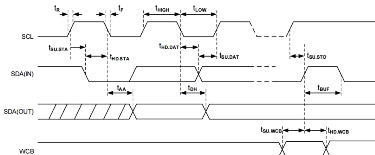
Figure 3-1 Bus Timing
