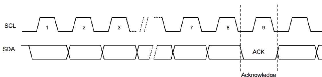
Figure 4-3 Output Acknowledge
