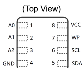
DFN-8 3*3/2*2
