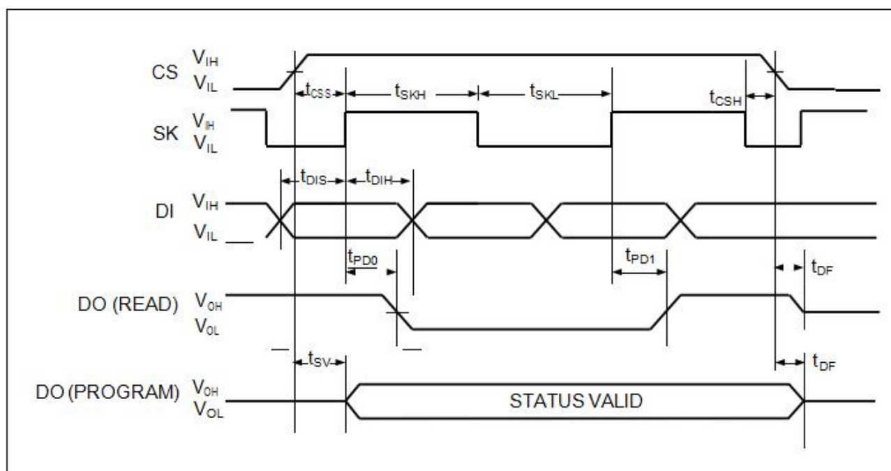
Figure 9 BUS Timing
