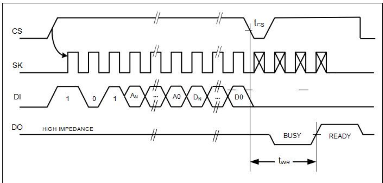
Figure 5 WRITE Timing
