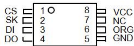
MSOP-8
