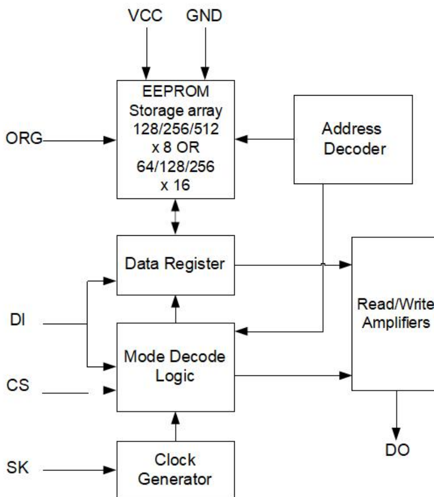
Figure 1 Block Diagram
