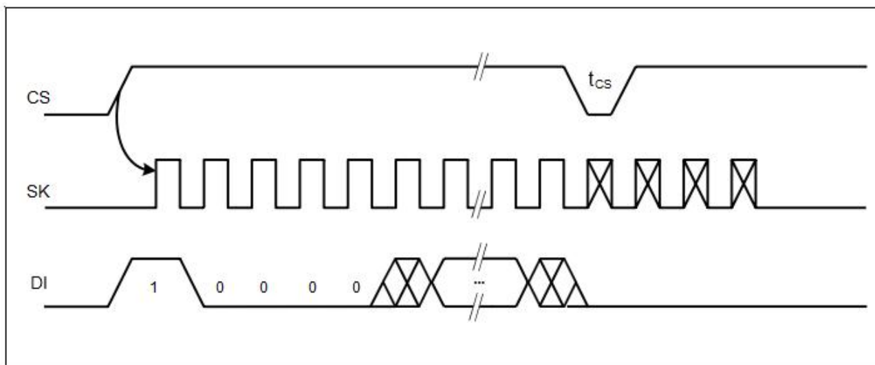
Figure 9 BUS Timing
