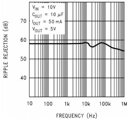
Figure 9. Ripple Rejection
