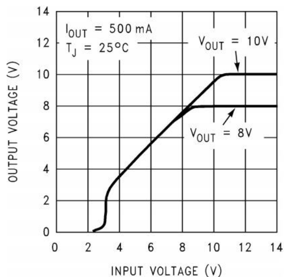
Figure 14. Low-Voltage Behavior
