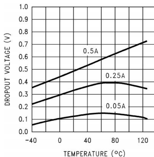
Figure 2. Dropout Voltage vs. Temperature
