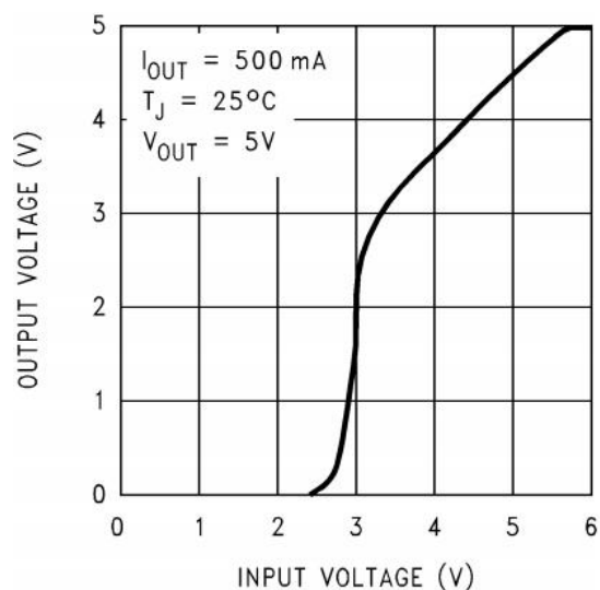
Figure 13. Low-Voltage Behavior
