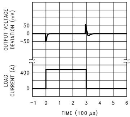
Figure 8. Load Transient Response
