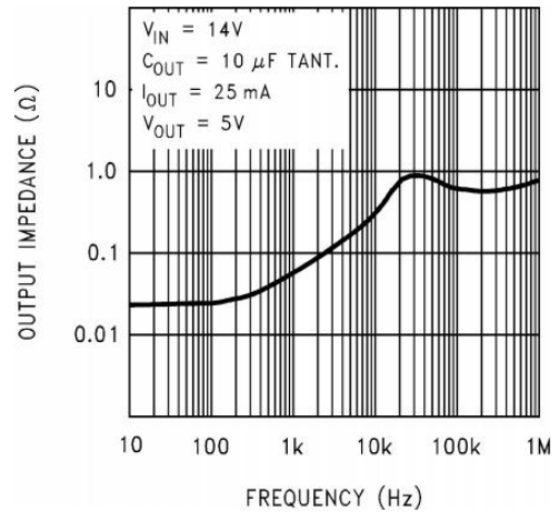
Figure 10. Output Impedance
