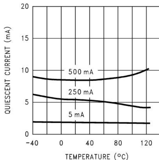
Figure 4. Quiescent Current vs. Temperature
