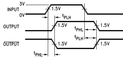
FIGURE 1. Propagation Delays
