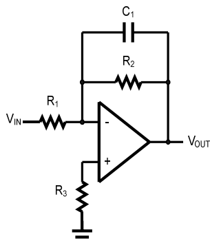
Figure 5. Low Pass Active Filter
