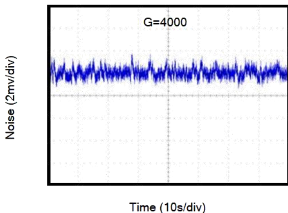
0.1Hz to 10Hz Noise at +5V
