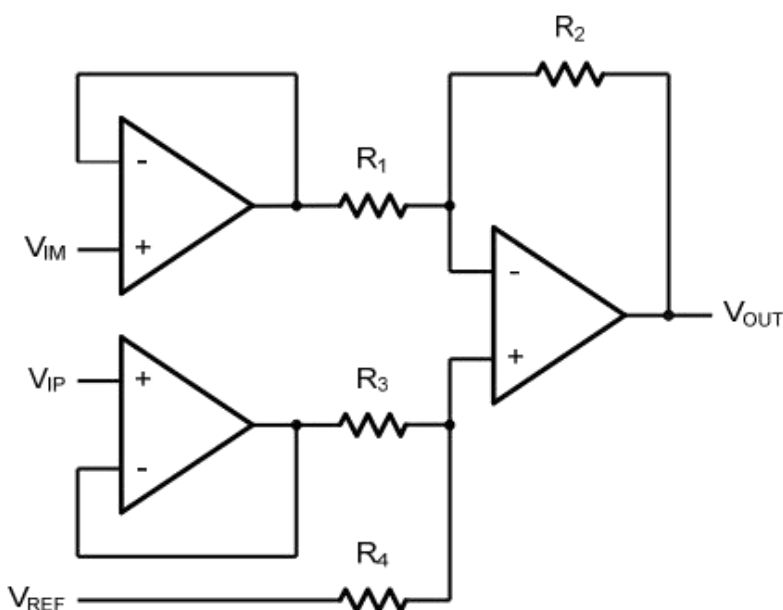
Figure 6. Instrument Amplifier
