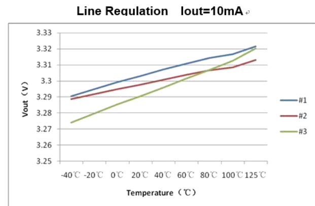
Output Voltage
