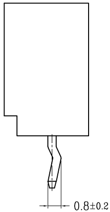
TYPE 2 (打K脚)
