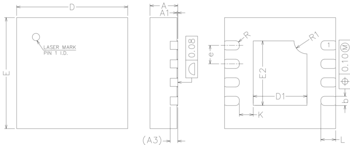
TOP VIEW
