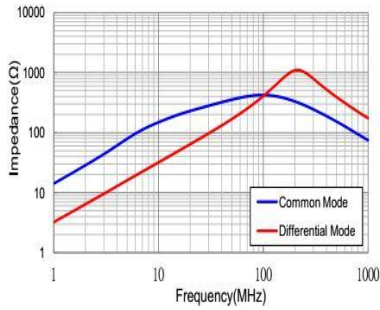
CM1513F-301-2P-T
