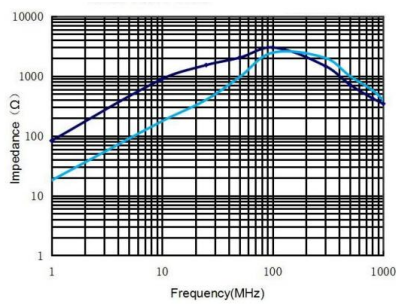
CMF9070F-501-2P-T
