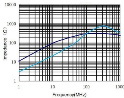
CMF9070F-132-2P-T
