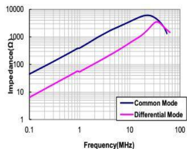
CM1211F-272-2P-T
