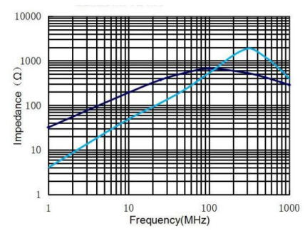
CMF9070F-302-2P-T
