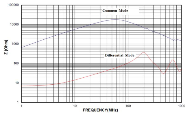
CMF3216F-602-2P-T
