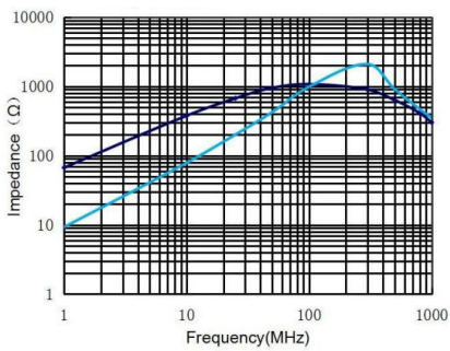
CM1211F-800-2P-T
