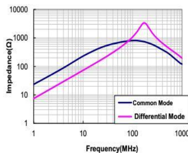
CM1211F-701-2P-T
