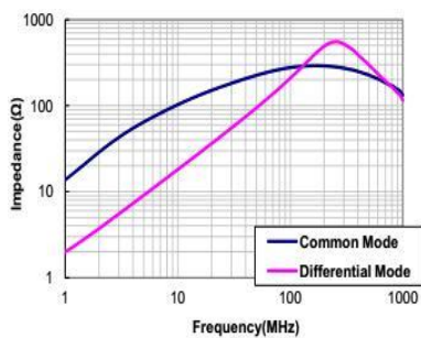
CM1211F-800-2P-T
