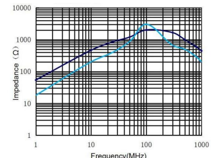
CM1211F-272-2P-T
