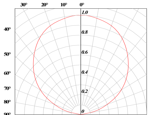
Radiation Pattern
