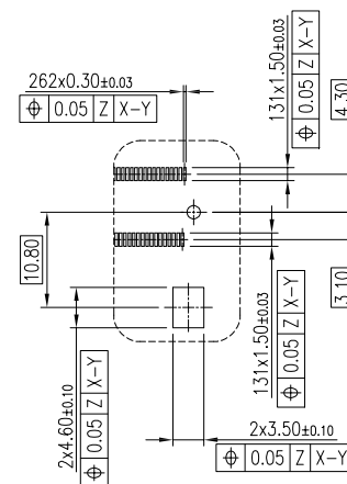
DETAIL H SCALE 1:1
