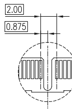
DETAIL F SCALE 2:1
