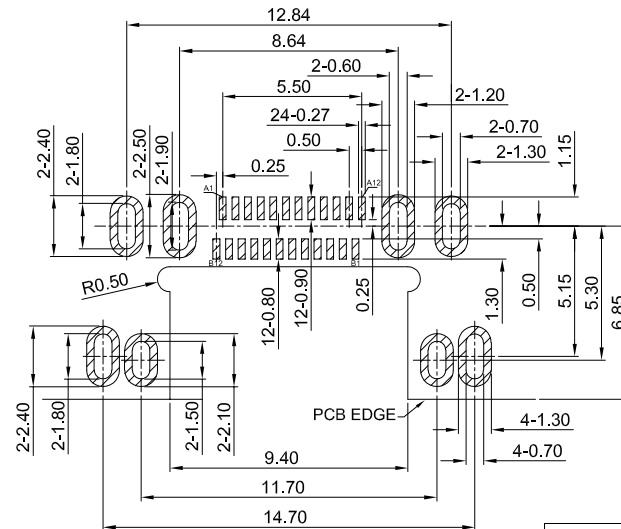
PCB REFERENCE DIAGRAM TOLERANCE: ±0.05
