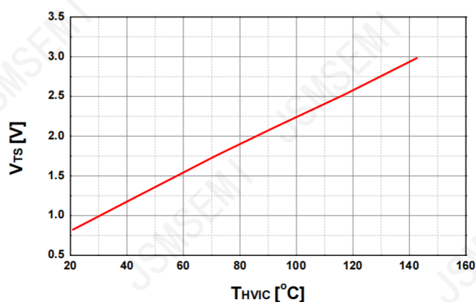
Figure 4. Temperature Profile of VTS(Typical)
