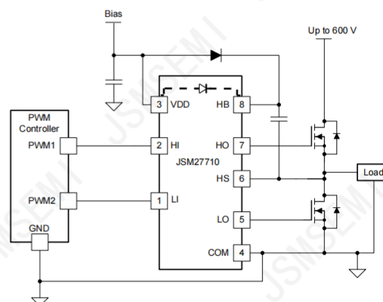
Simplified Schematic
