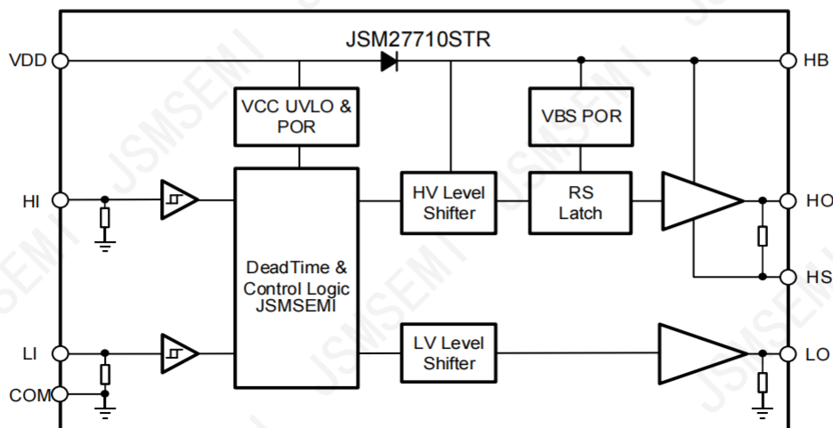
Figure 2. JSM27710 Block Diagram
