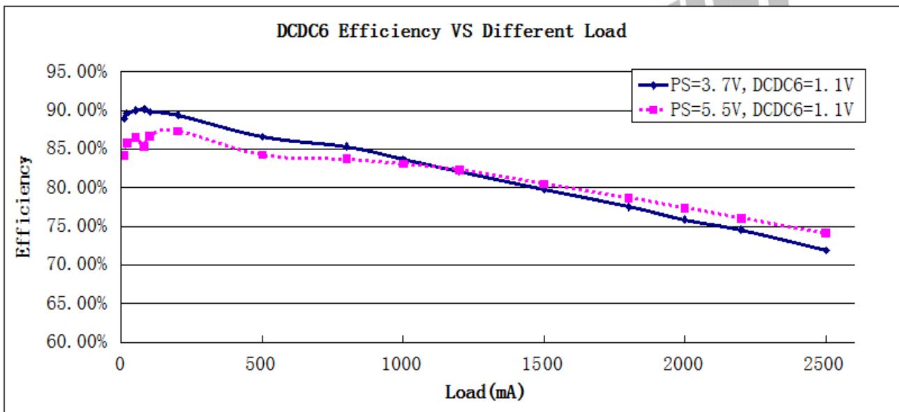
Figure 6-6 DCDC6 Efficiency VS Different Load
