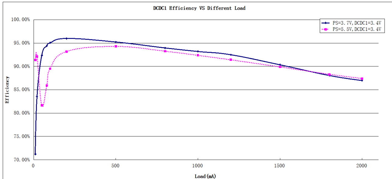
Figure 6-1 DCDC1 Efficiency VS Different Load
