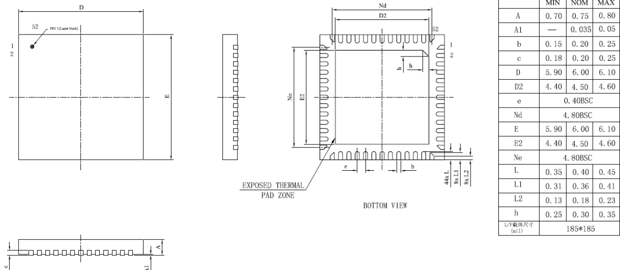
Figure 10-1 Package Information
