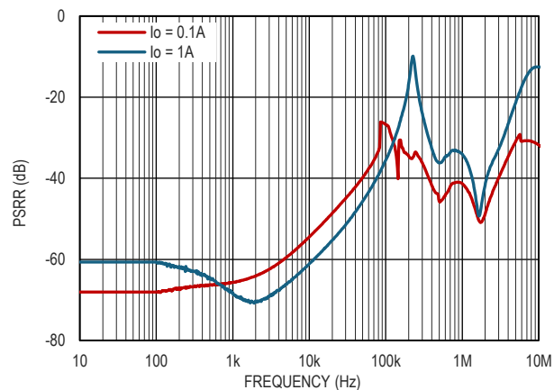
图 12. PSRR, V_{IN} = 5V , V_{OUT} = 3.3V
