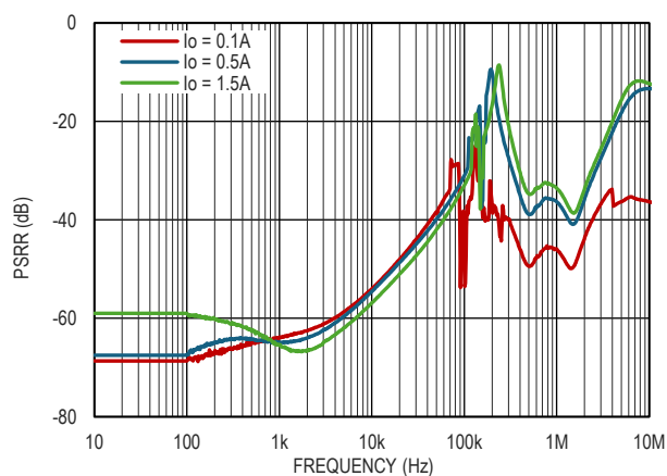
图 13. PSRR, V_{IN} = 3.8V , V_{OUT} = 3.3V
