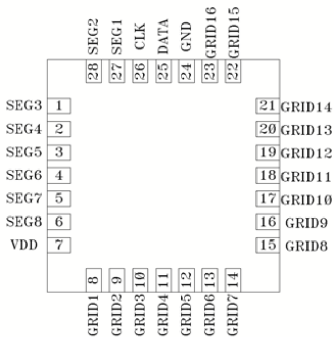
QFN28
