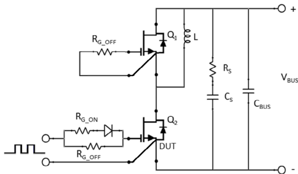
Figure 22. Schematic of the Half-Bridge Mode Switching Test Circuit. A Bus RC Snubber ( R_S = 2.5\text{ }\Omega , C_S = 100\text{ nF} ) is Used to Reduce the Power Loop High Frequency Oscillations
