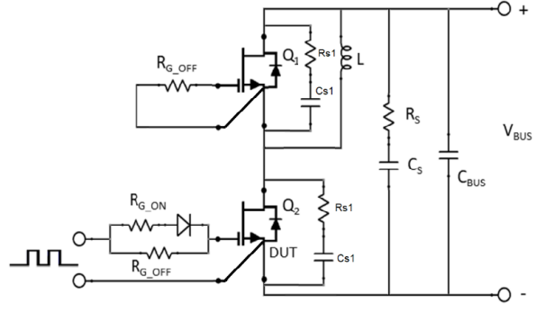
Figure 23. Schematic of the Half-Bridge Mode Switching Test Circuit with Device RC Snubber ( R_{S1} = 5\text{ }\Omega , C_{S1} = 95\text{ pF} ) and a Bus RC Snubber ( R_S = 2.5\text{ }\Omega , C_S = 100\text{ nF} )
