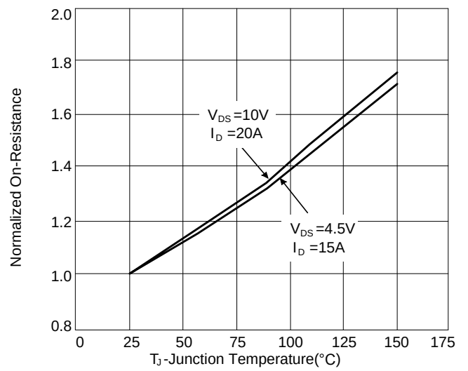
Figure 2: Rdson-Junction Temperature
