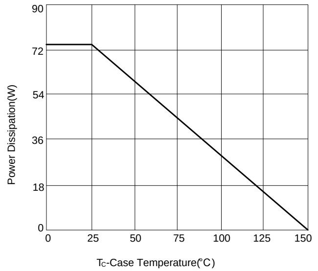
Figure 8: Power De-rating
