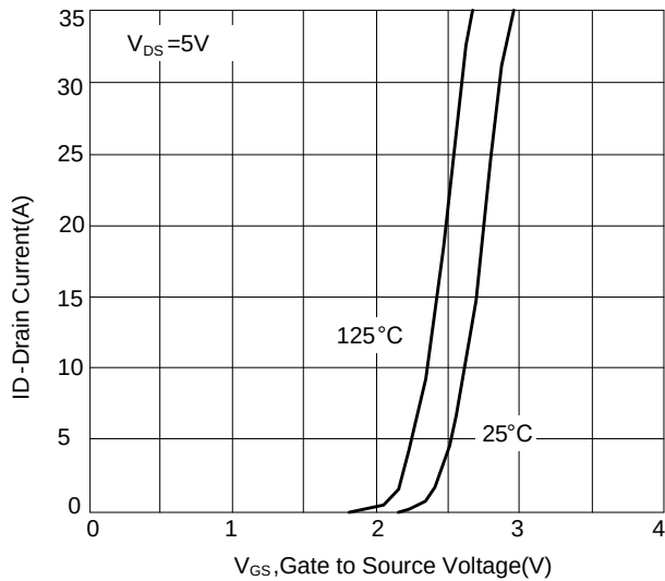
Figure 3: Transfer Characteristics
