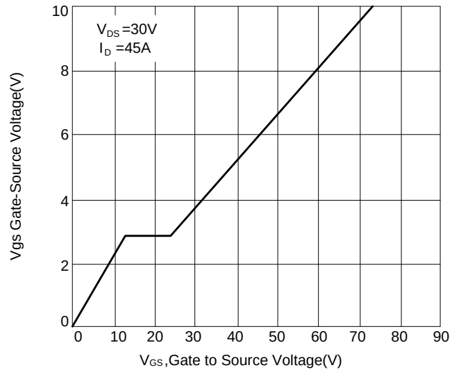
Figure 4: Gate Charge
