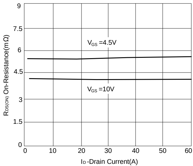
Figure 5: Rdson-Drain Current
