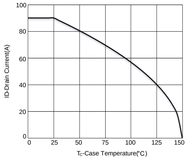
Figure 10: Current De-rating
