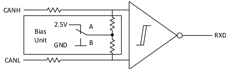
Figure 7-2. Bus States (Physical Bit Representation)
