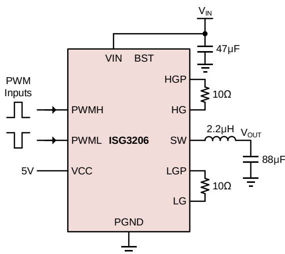
36V – 80V Input, 12V Output, and 200W Buck Converter
