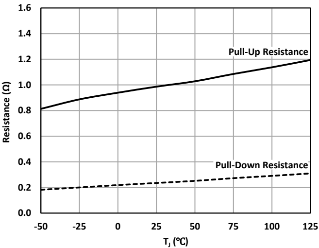
Figure 20. Output Pull-Down/Pull-Up Resistance vs Temperature
