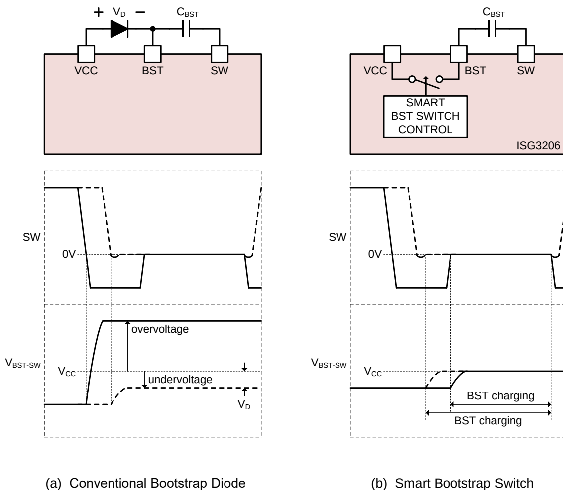
Figure 27. Operation Principle of Bootstrap Supply
