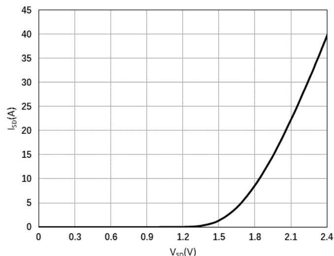
Figure 3. Source-Drain Reverse Conduction Voltage (25°C)
