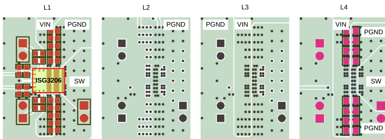
Figure 28. Four-Layer Layout Example
