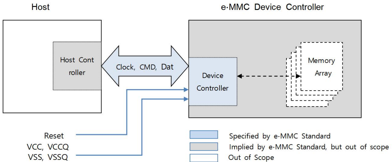
Figure 2 - e-MMC System Overview
