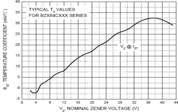
Temperature Coefficients
