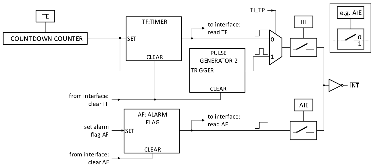
Fig 6. Interrupt scheme
