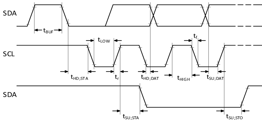
Fig 1. I²C-bus timing waveforms
