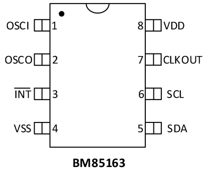
Pin Functions
