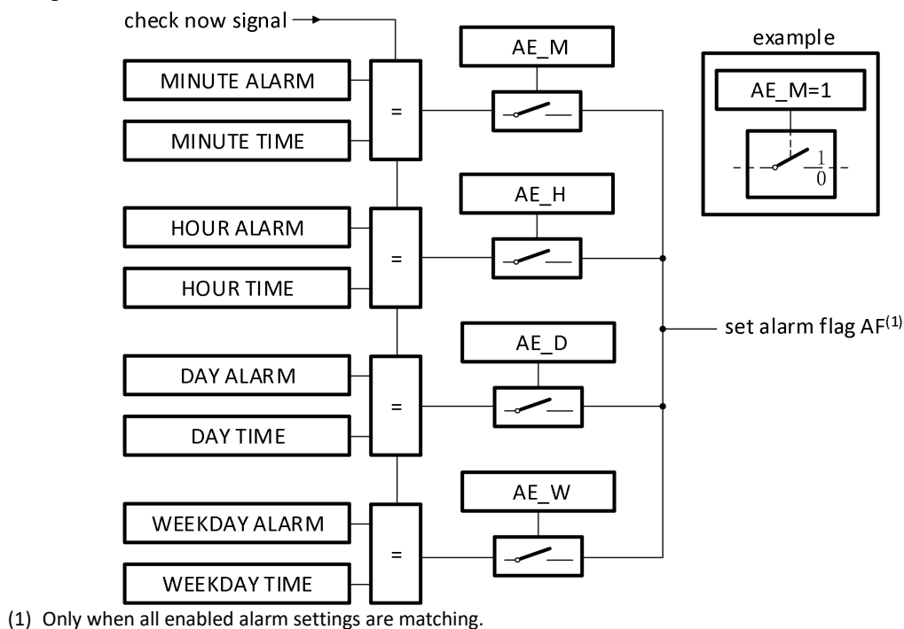
Fig 10. Alarm function block diagram
