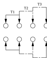
SCHEMATIC(SHORTING)
