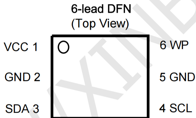
Figure 1: Package types
