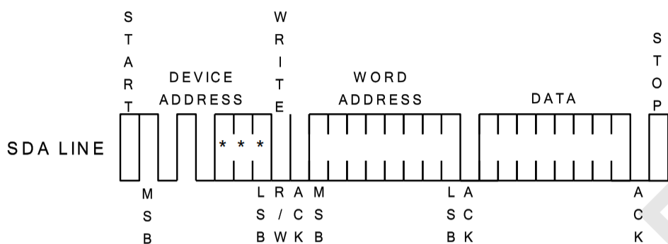
Figure 5: Byte Write
