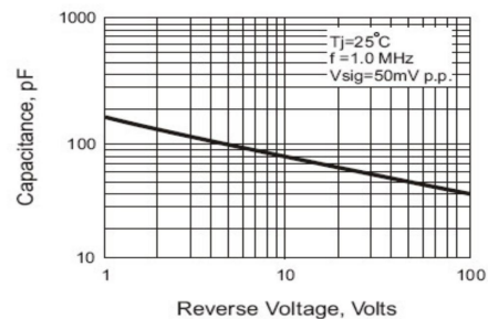
Fig. 5 Typical Junction Capacitance
