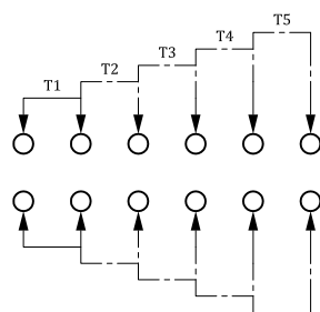
SCHEMATIC(SHORTING)
