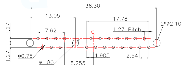
RECOMMENDED PCB LAYOUT PCB TOLERANCE:±0.05
