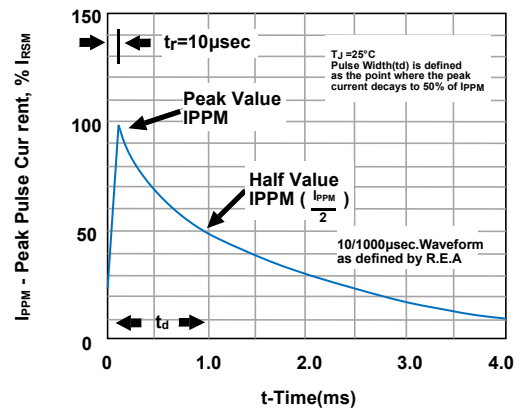
Figure 4 - Pulse Waveform
