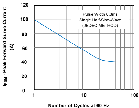
Figure 7 - Maximum Non-Repetitive Surge Current
