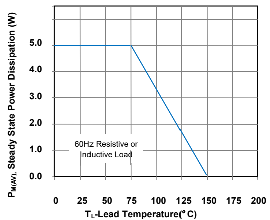
Figure 6 - Steady State Power Derating Curve
