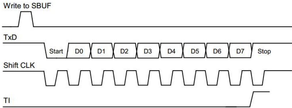
Figure 15-2 Send Timing of Mode 1
