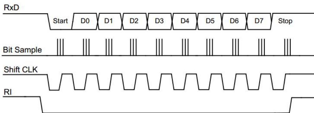
Figure 15- 3 Receive Timing of Mode 0
