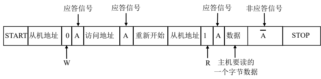
Figure 17-8 主机向从机读写数据 1 个字节数据
